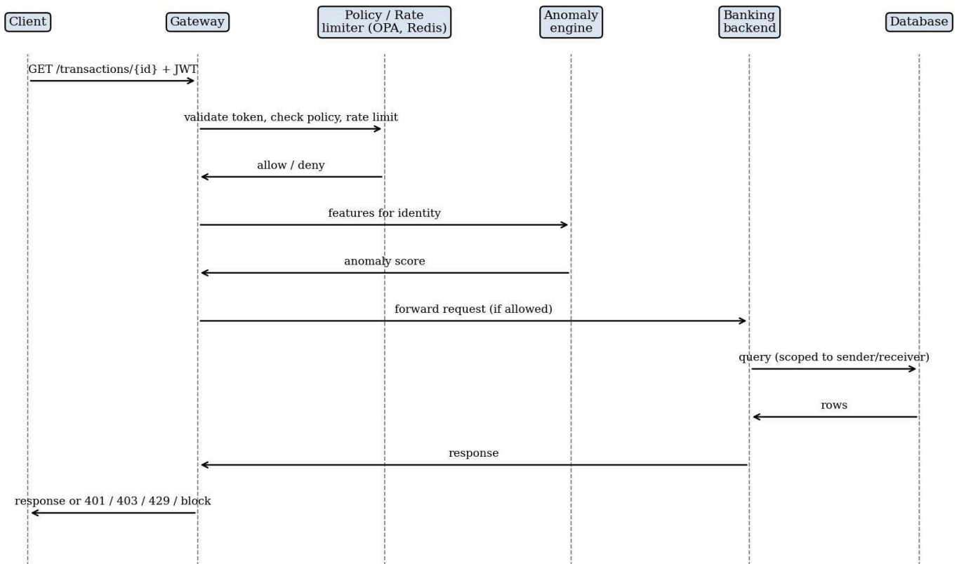
Figure 3.4 Sequence diagram for a request through the gateway
