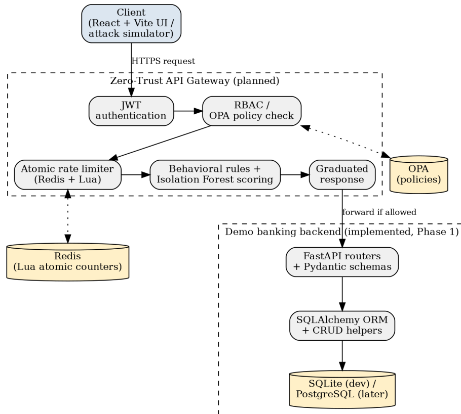
Figure 3.1 System architecture of the Zero-Trust API Gateway
