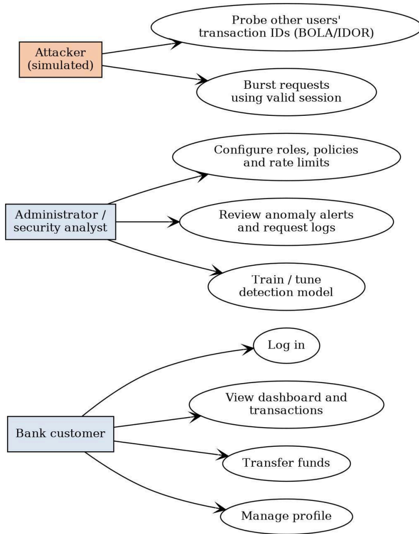
Figure 3.2 Use case diagram
