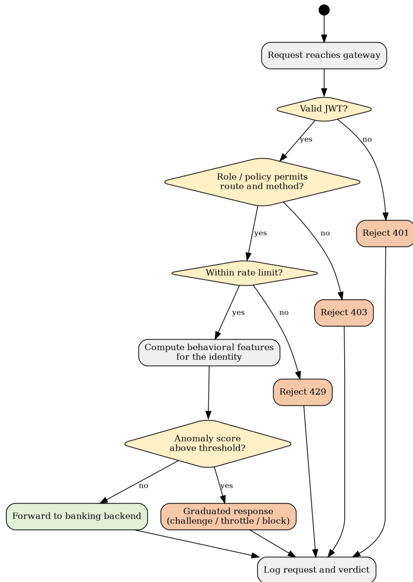
Figure 3.3 Activity diagram of a single request
