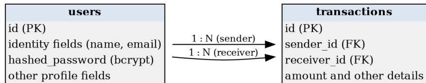
Figure 4.1 Data model of the banking backend
